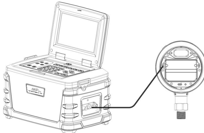
Figure 11 Barometric calibration
