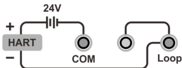
Figure 8 HART-External power and internal resistance
