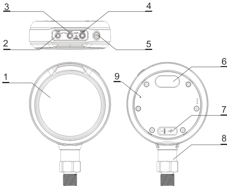
Figure 1 Basic Structure
