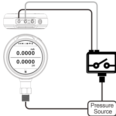
Figure14 Calibrate Pressure Switch
