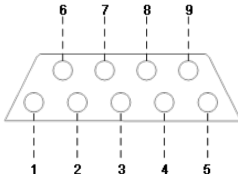
Figure 18 Description of RS232 module DB9 female pins
