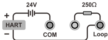
Figure 9 HART-External power and external resistance
