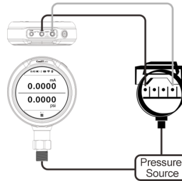
Figure 13 Calibrate pressure transmitter
